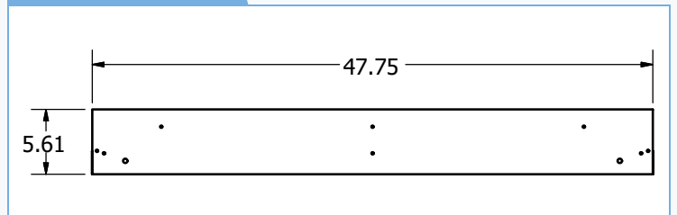
2x4 End Dimensions
